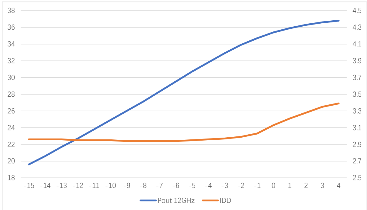
Pout and IDD vs Pin at 12GHz
